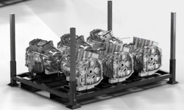
> K35 Size 1478 x 1136 x 774 mm max load 500 kg levels 3
